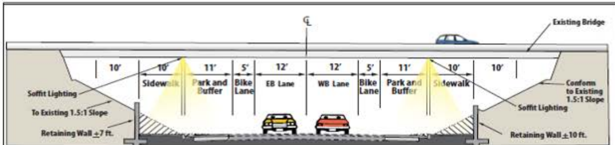
Chestnut Ave. Undercrossing Facing West Typical Cross Section
